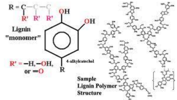
Lignin chemistry
